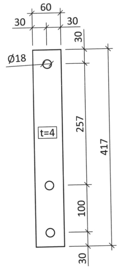
FESTING F2 M1:5
