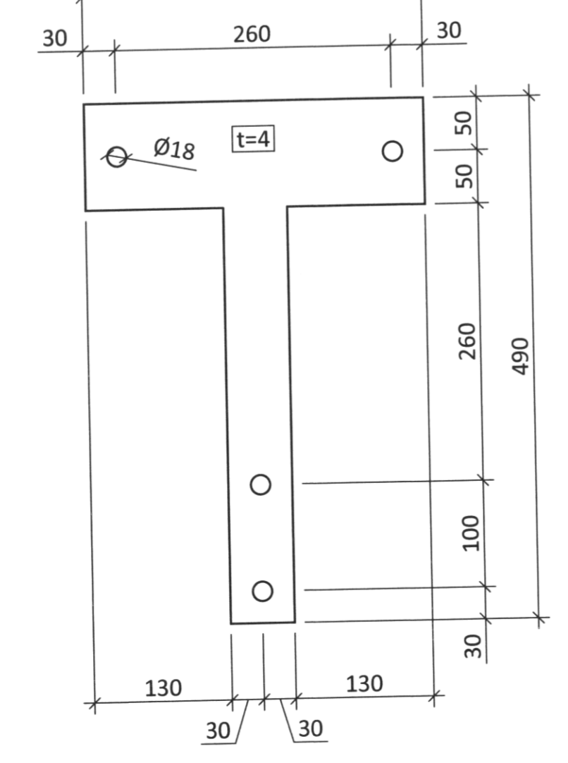
FESTING F3 M1:5
