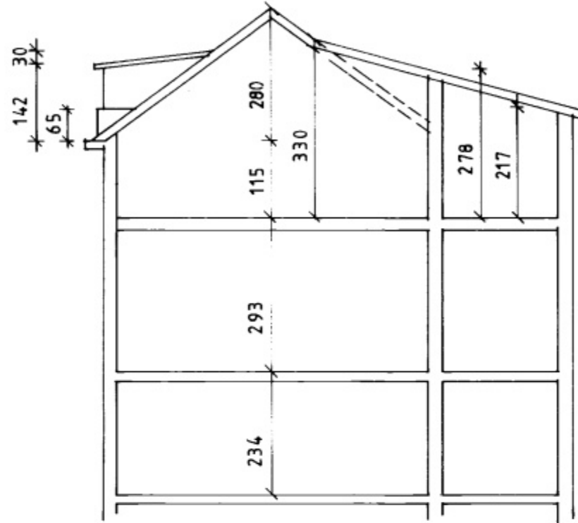
SNID B-B
