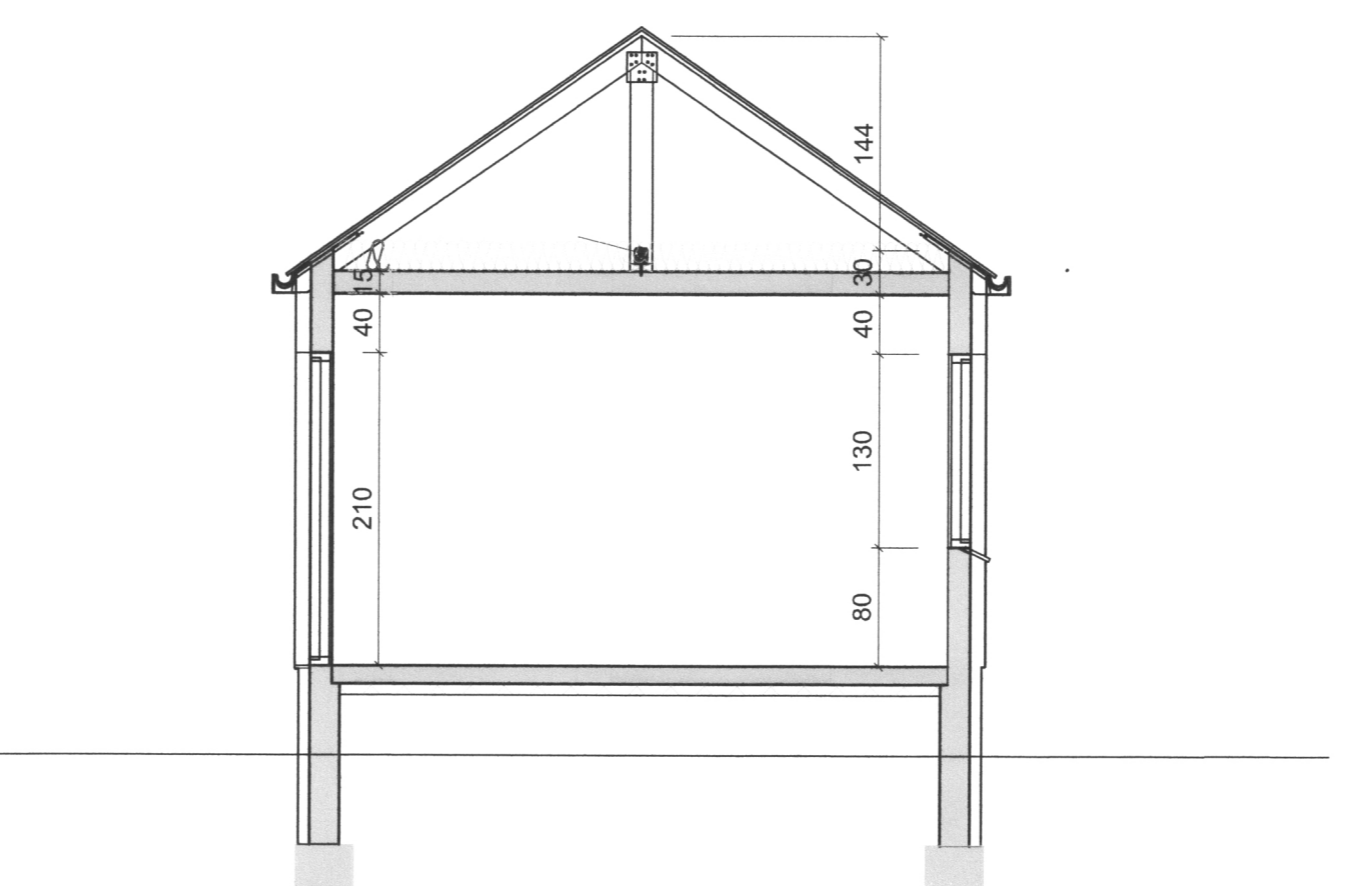
SNID B-B
