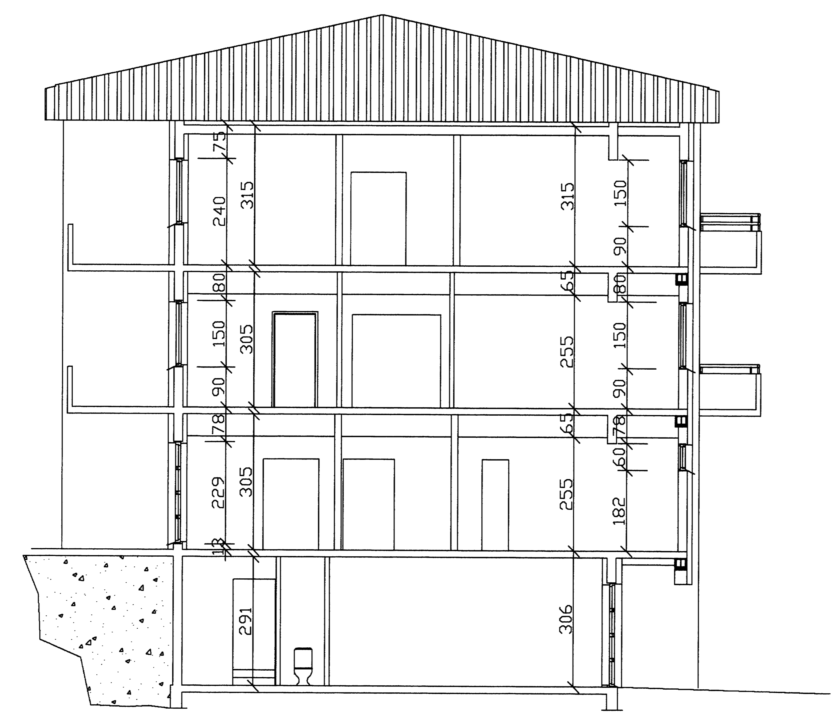
SNID C-C
