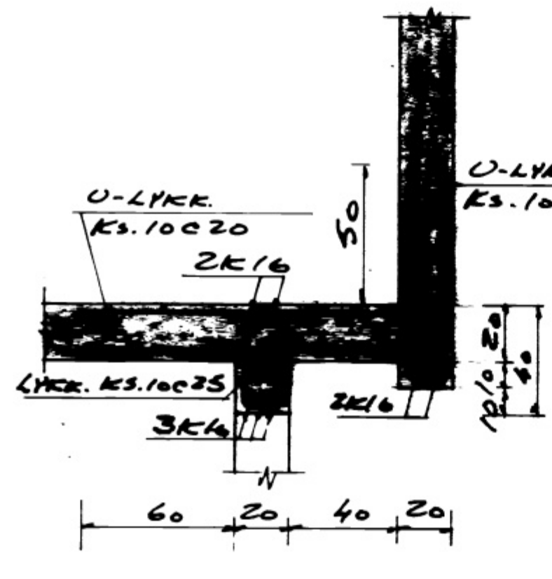
SNID E-E 1:20
