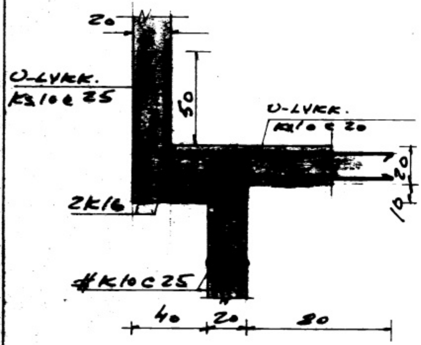
SNID F-F 1:20
