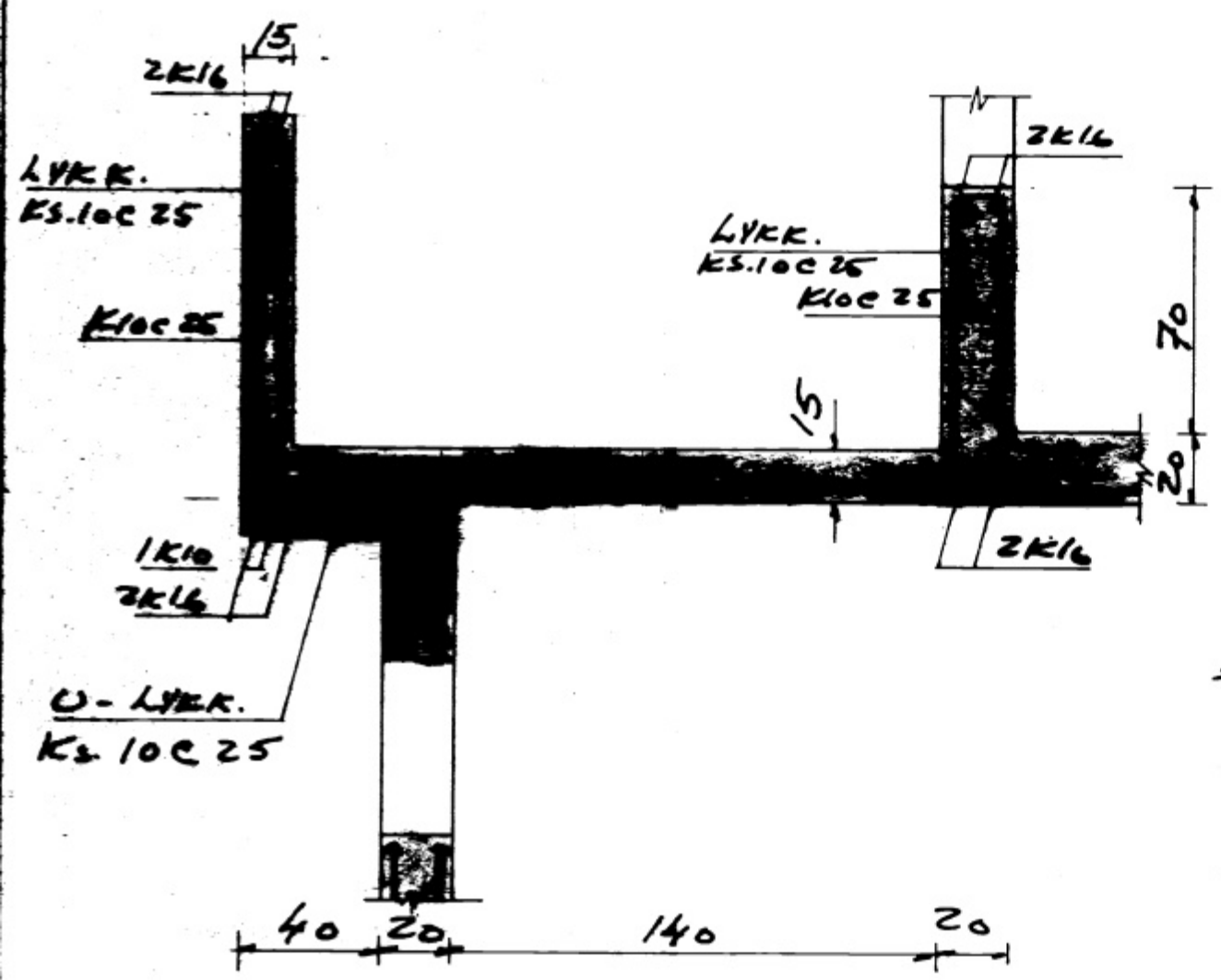
SNID F-F 1:20
