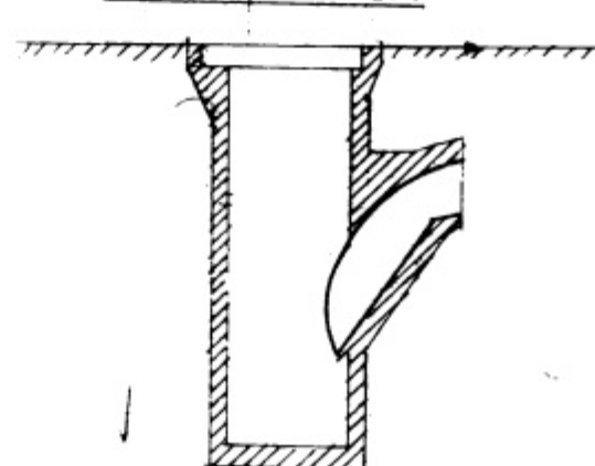
SANDFANG (SF)
