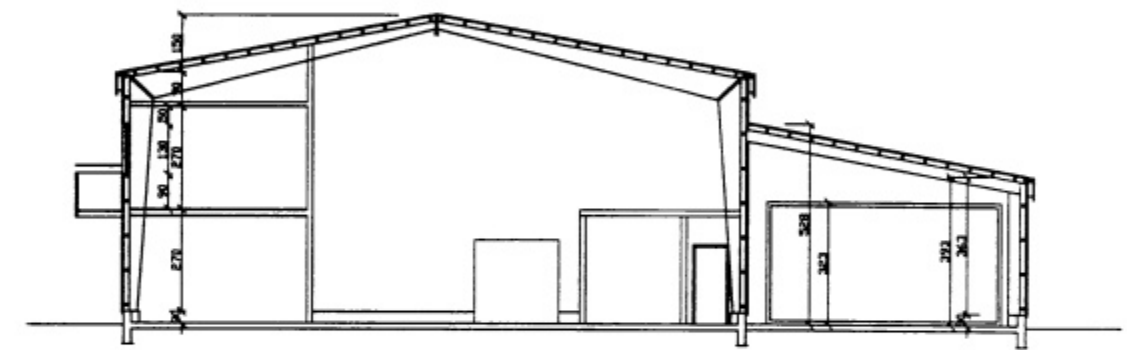
SNID B-B
