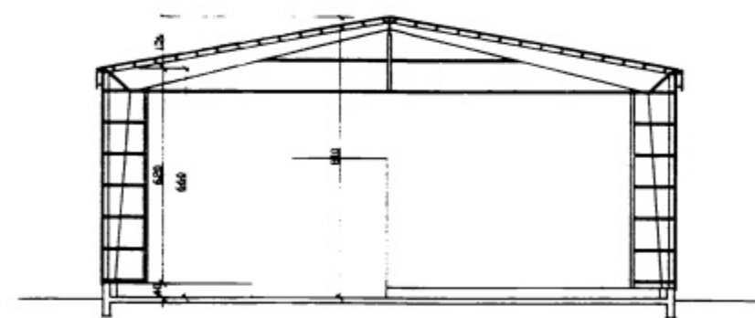
SNID C-C
