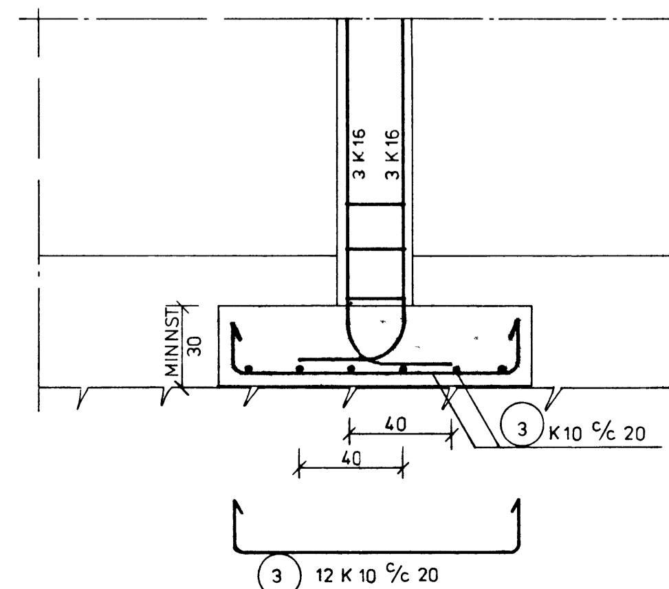
SNID D-D, M 120
