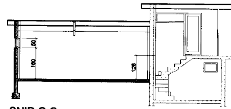
SNID C-C
