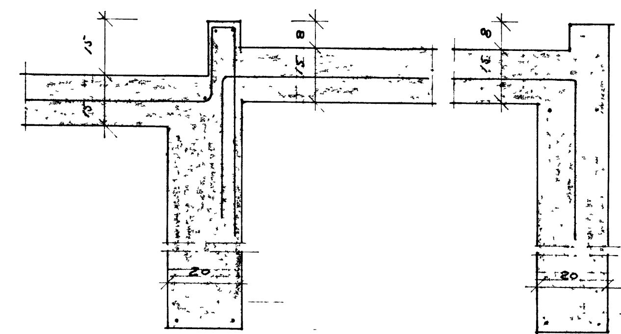
SNID C-C 1/10
