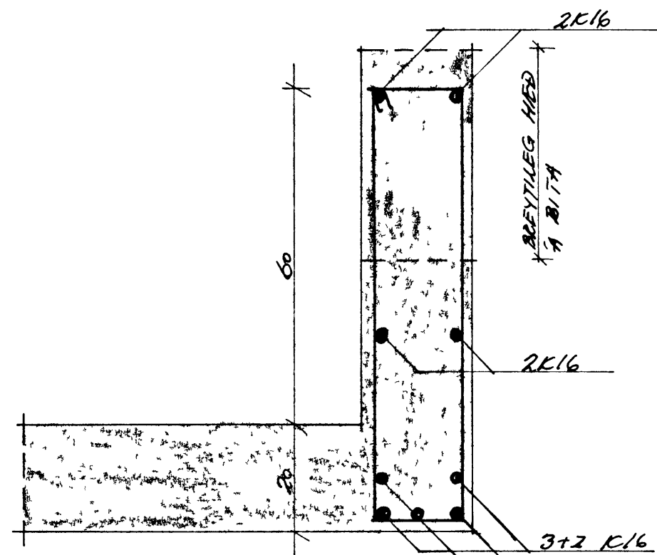
SNID C-C 1:10
