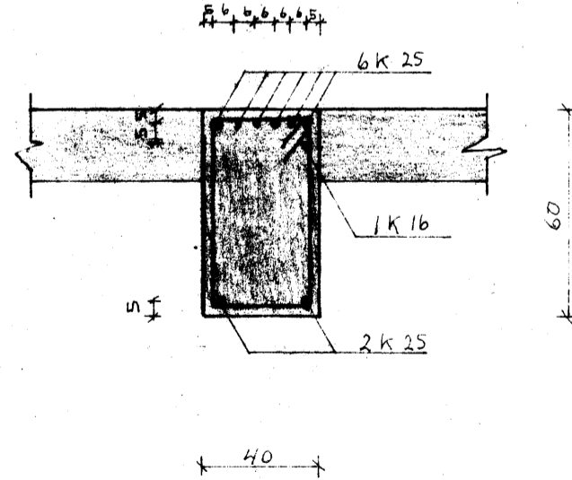
SNID B-B Mkv 1:20
