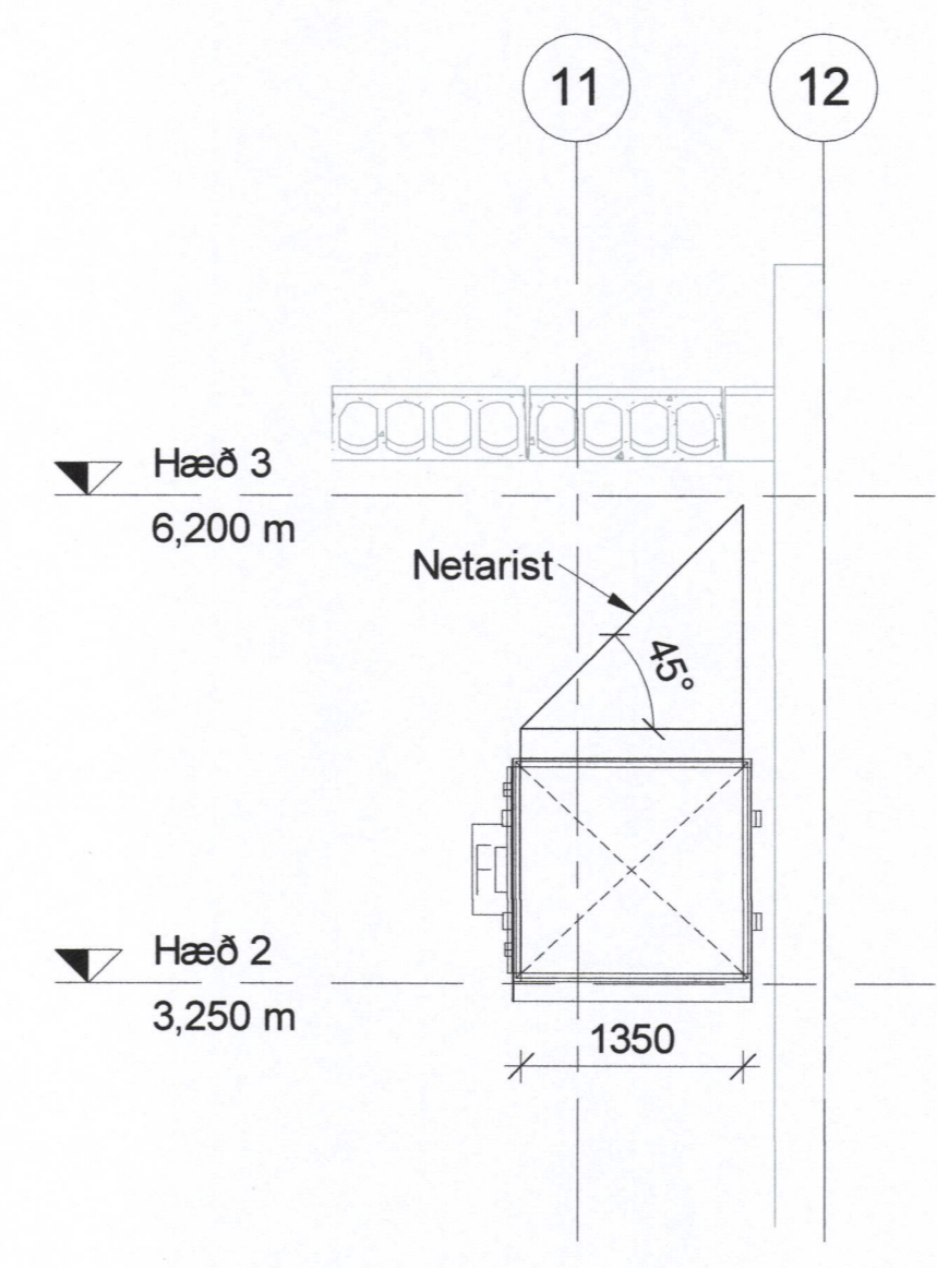
C SNID M47.202 1 : 50
