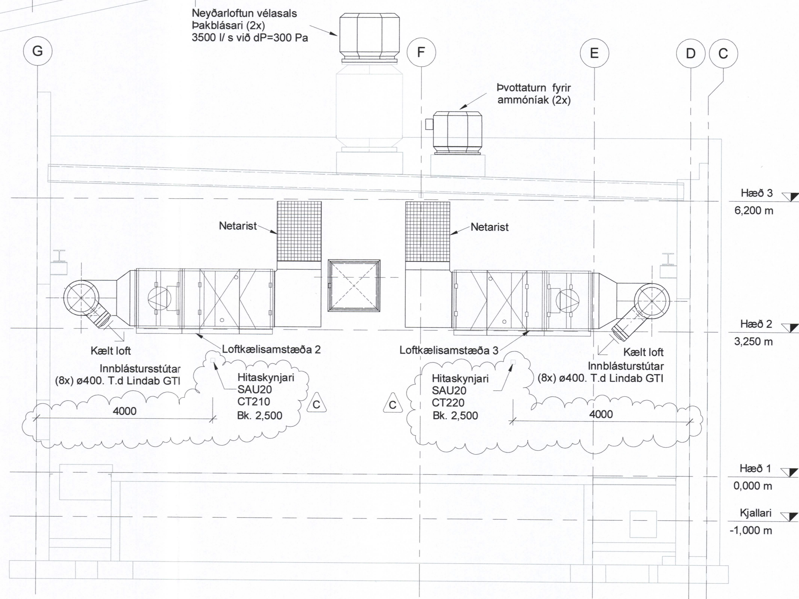
B SNID M47.202 1 : 50
