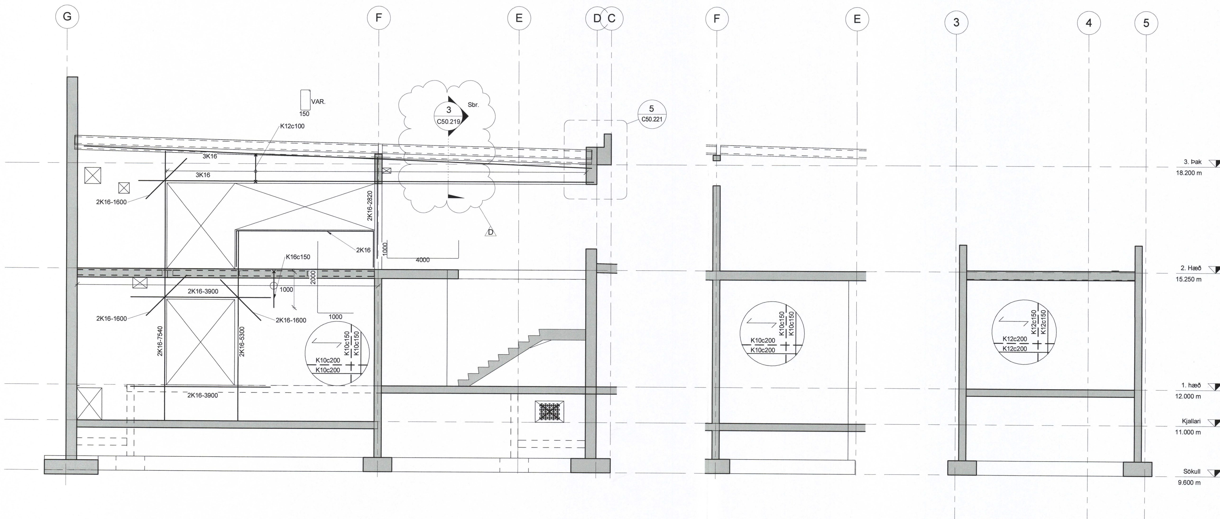
1 SNID C50.203 1:50
