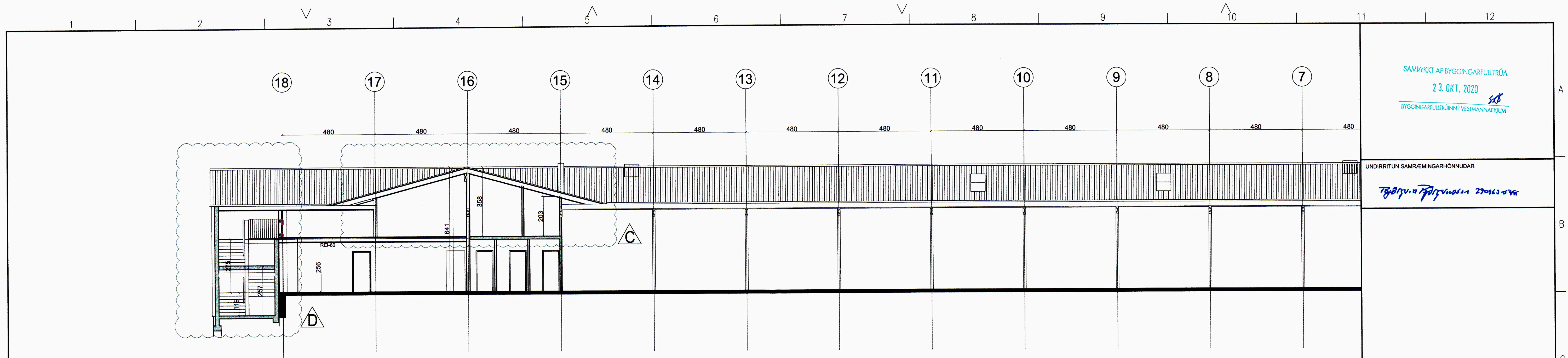
SNID E-E 1:100
