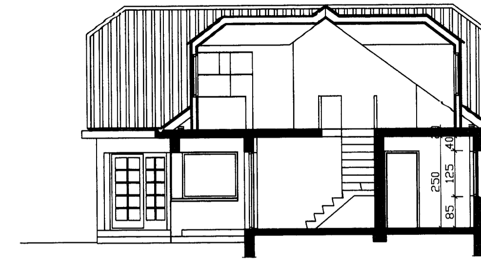
SNID B-B
