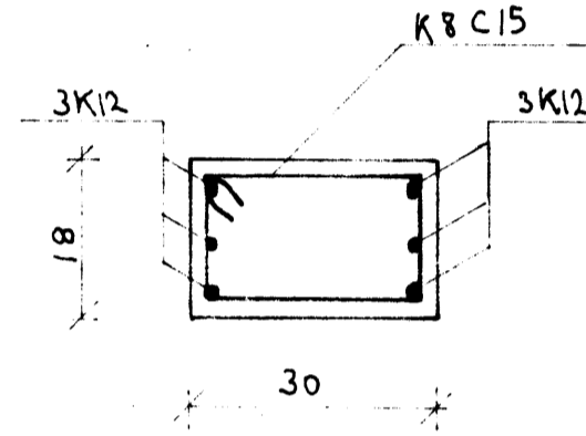
SNID B-B MKV 1:10
