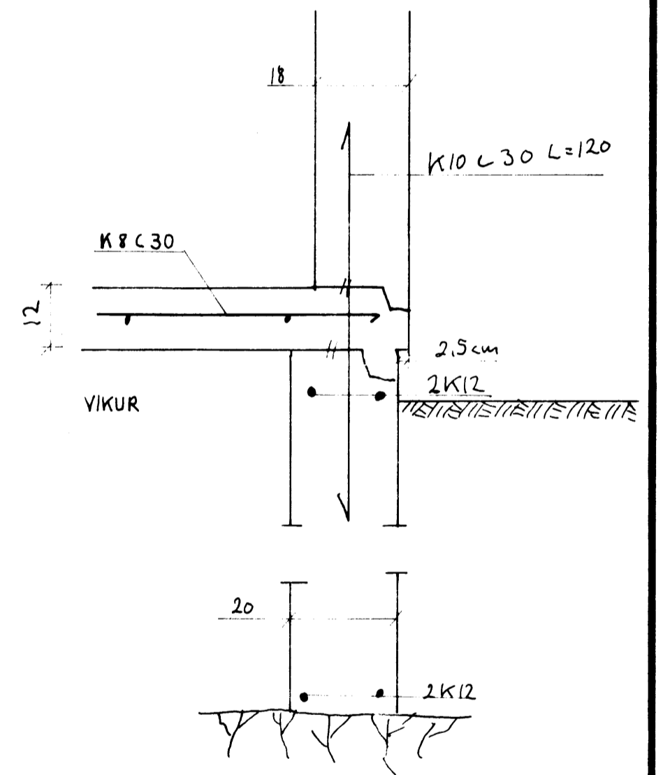
SNID 'I' UNDIRSTÖÐUR MKV 1:10
