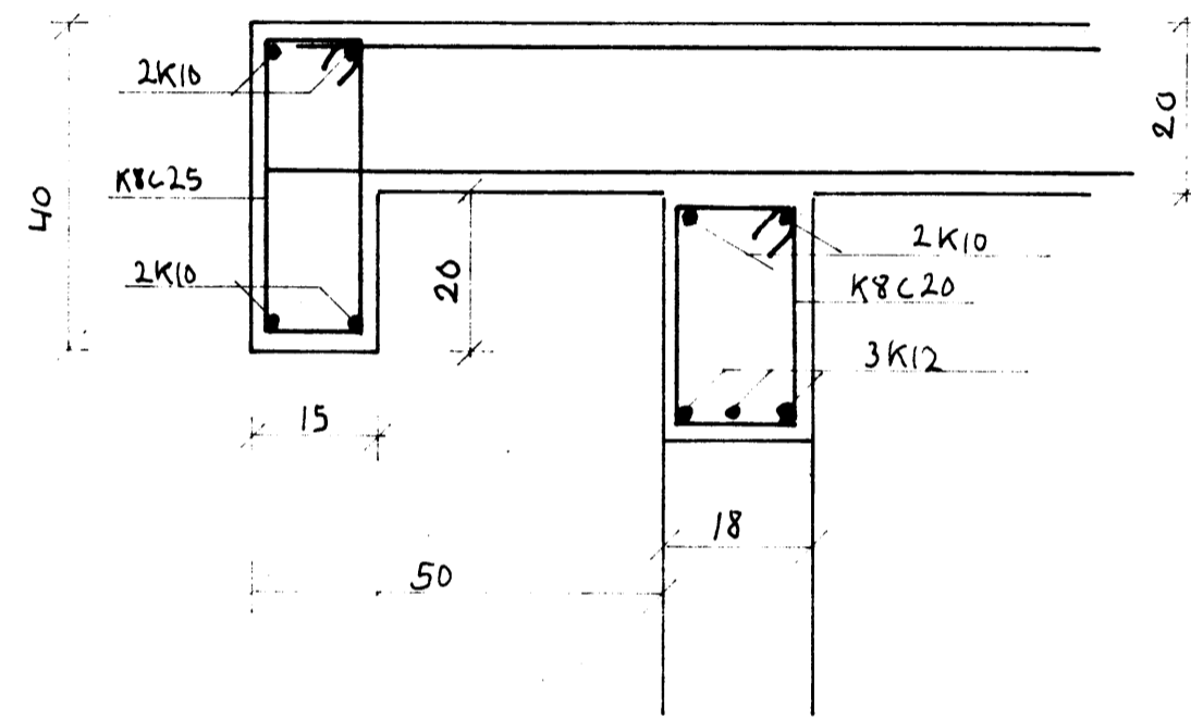
SNID C-C MKV 1:10
