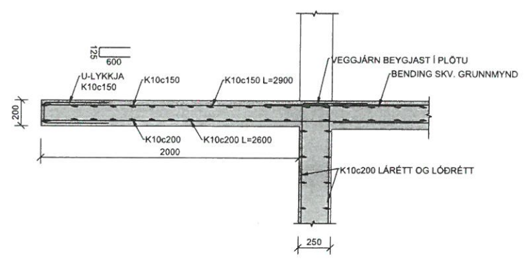
B SNID 1:20
