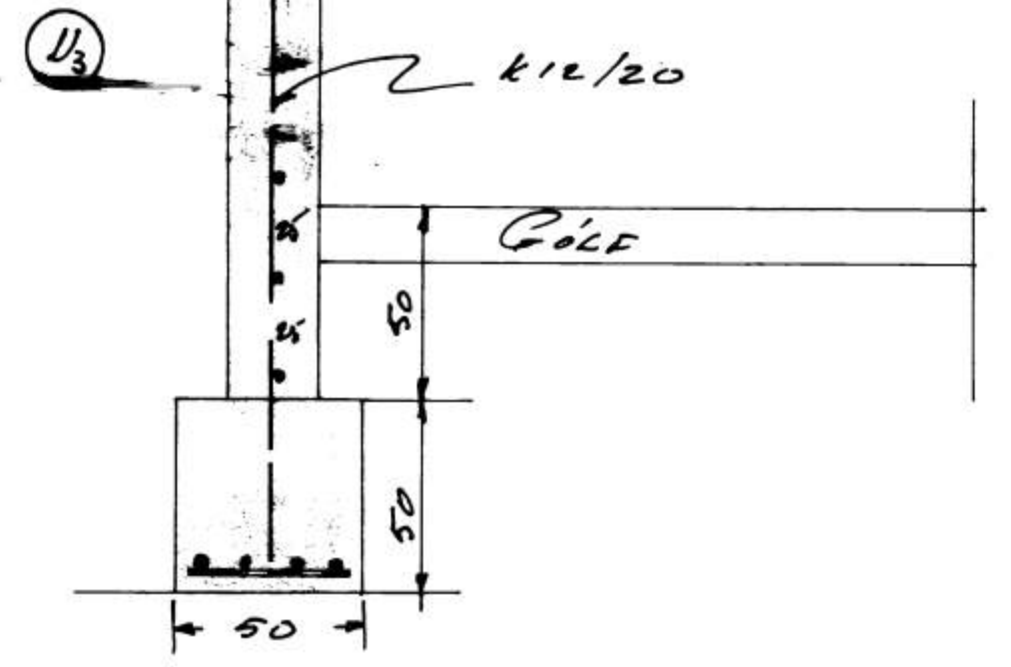
UNDIRSTAÐA 1:20 4 K12 LANGS K12/25 ÞVAGET.
