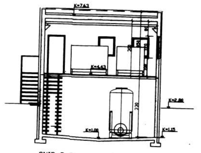
SNID B-B
