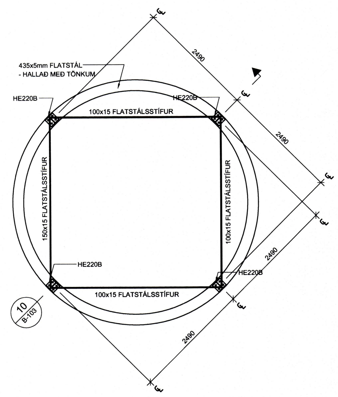
SM1 SNID 1:10
