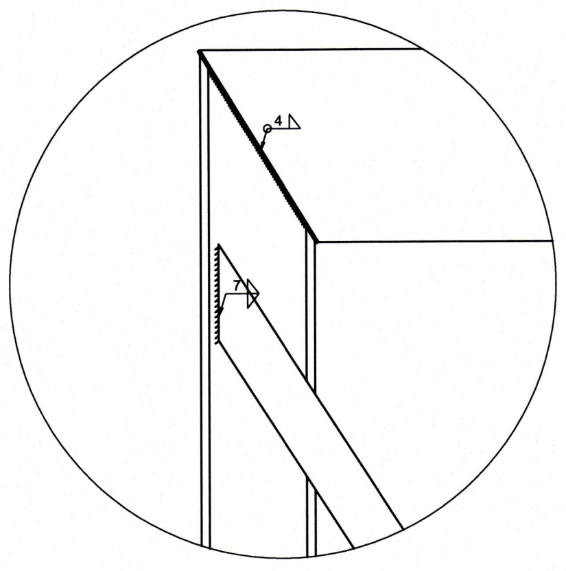
SM2 SNID 1:10
