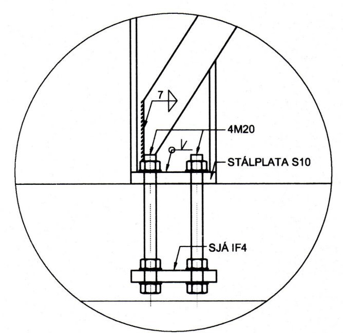
SM1 SNID 1:10
