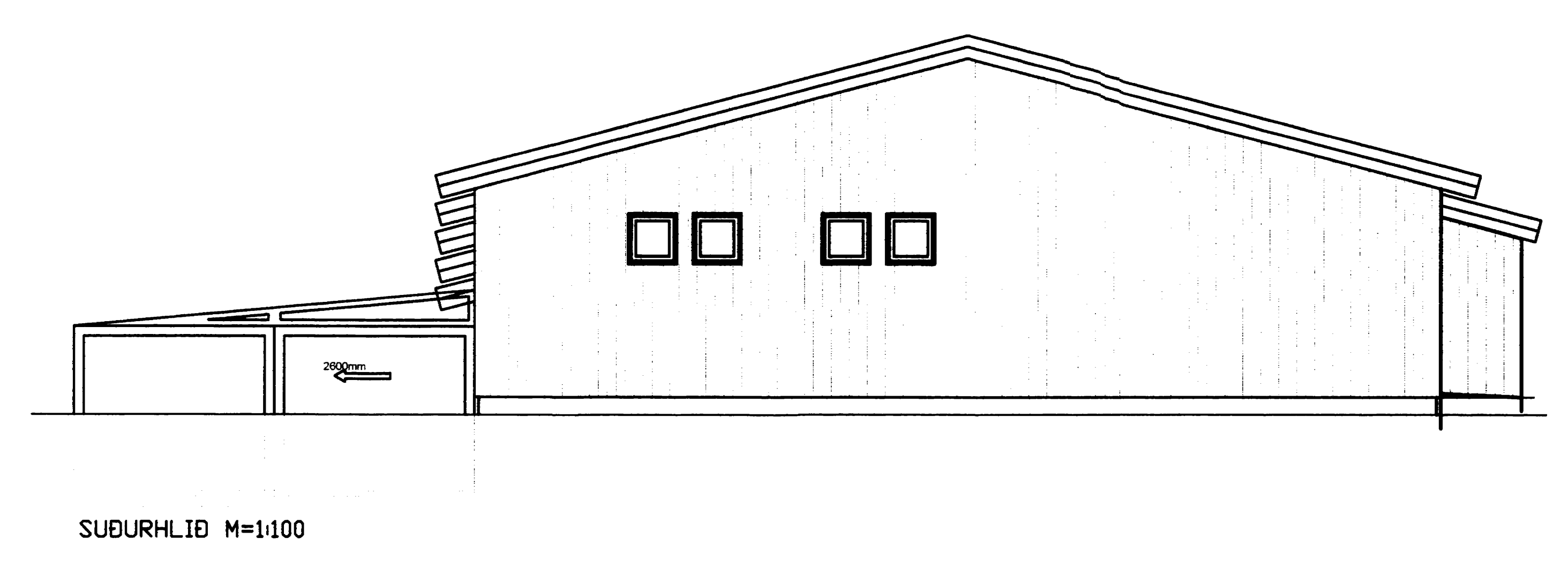
SUBURHLID M=1:100
