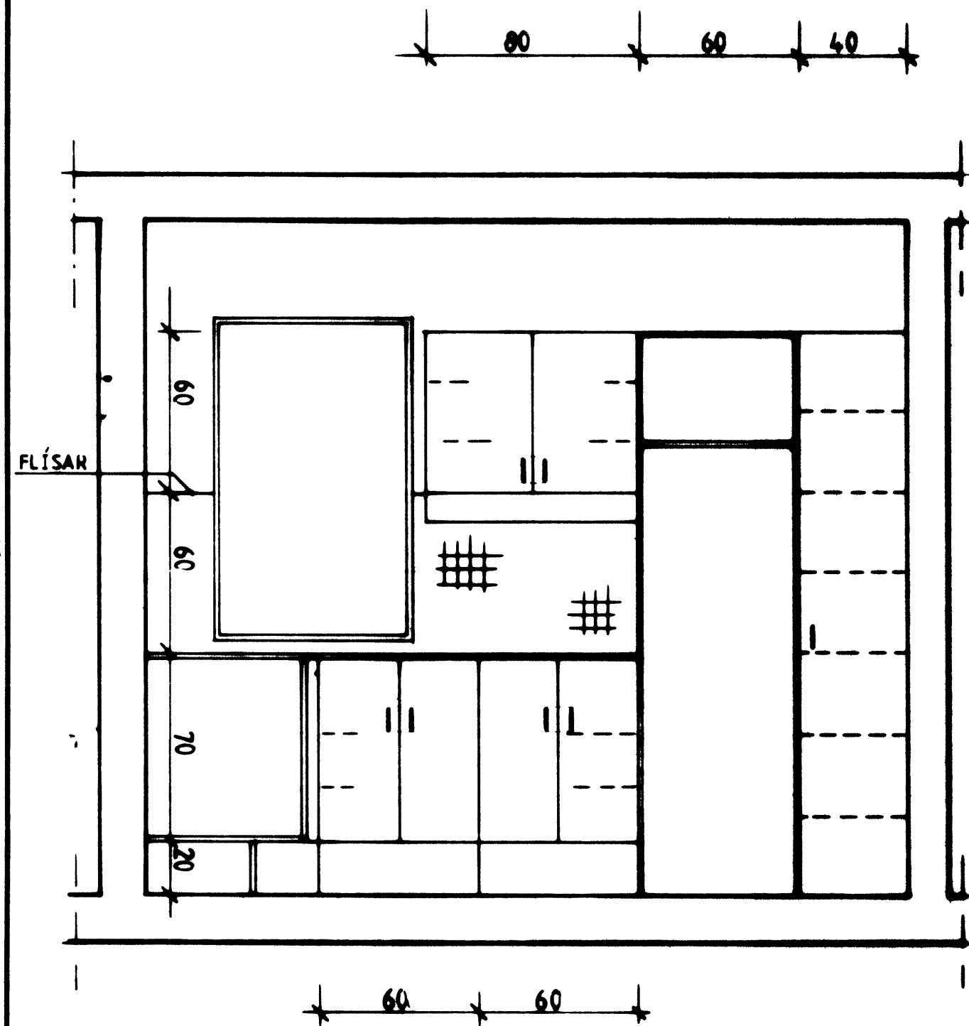
SNID B-B
