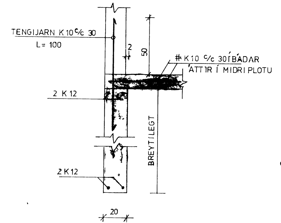
SNID E-E MKV 1:20
