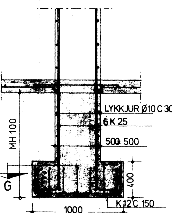
SNID-D-1:20
