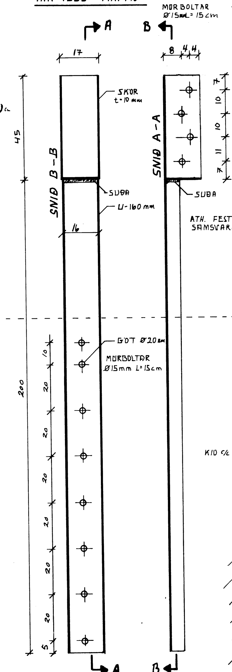
FESTING LÍMTRES VÍÐ INN VEGB MKV 1:10
