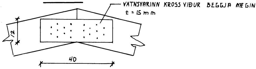
FESTING LÍMTRES VÍÐ INN VEGB MKV 1:10
