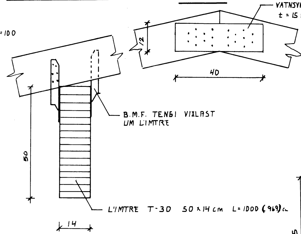
FESTING LÍMTRES VÍÐ SPERRUR MKV 1:10
