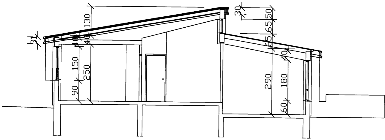
SNID
