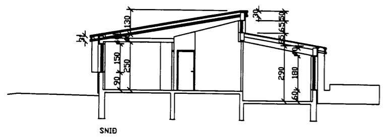
SNID
