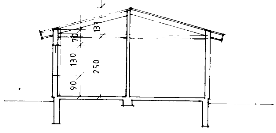
SNID B-B 1100
