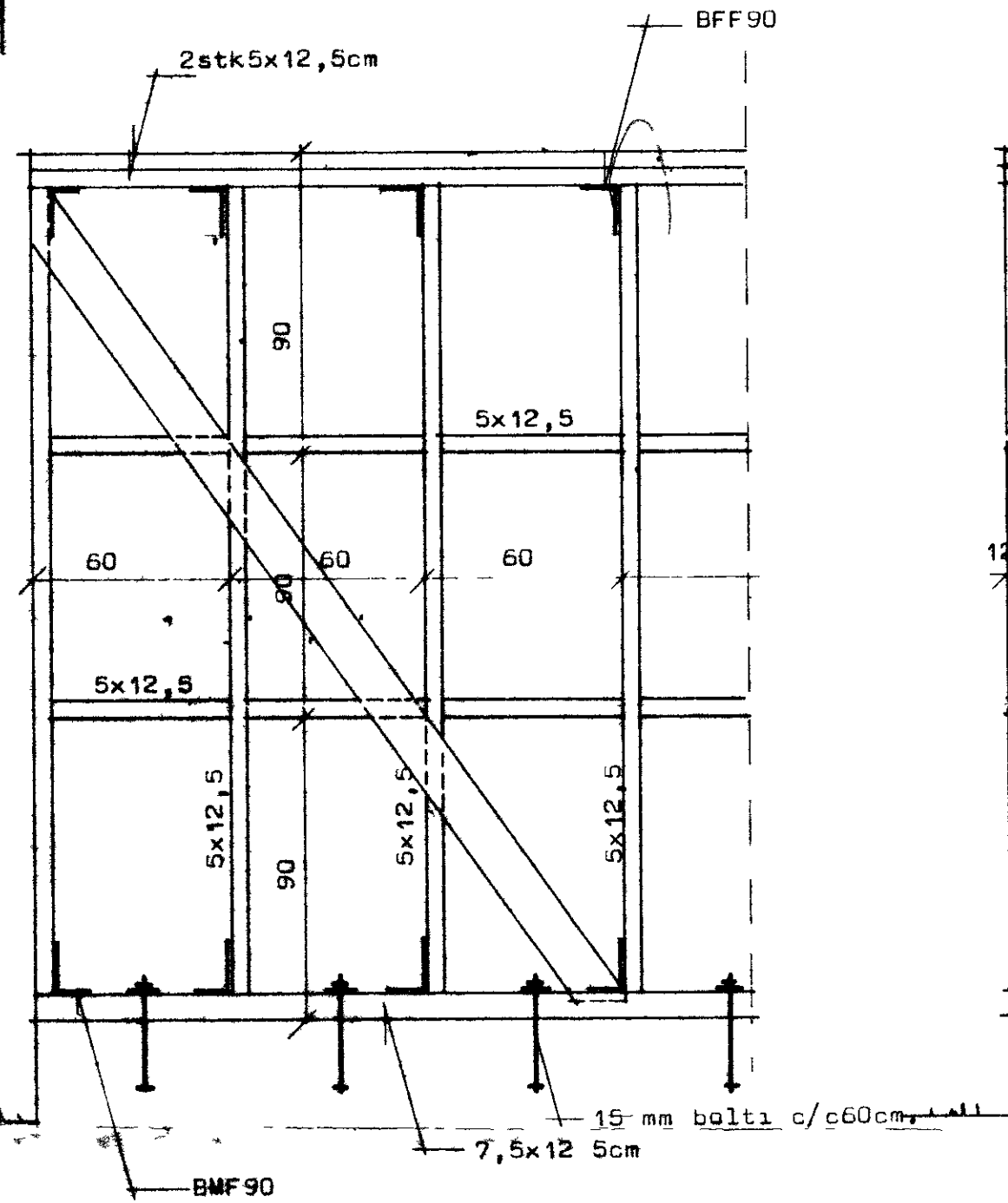
Fragangur a horni
