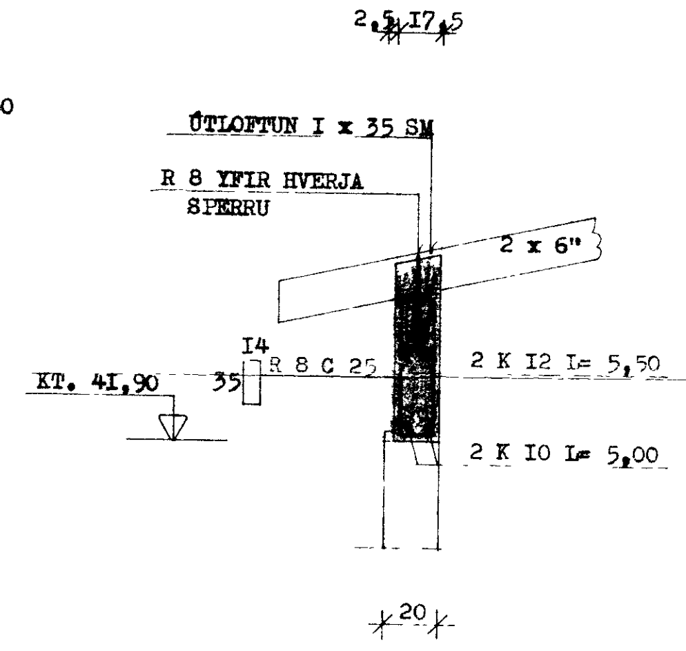
SNID C - C 1:20
