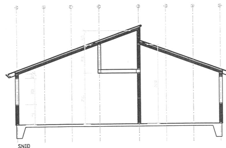
SNID
