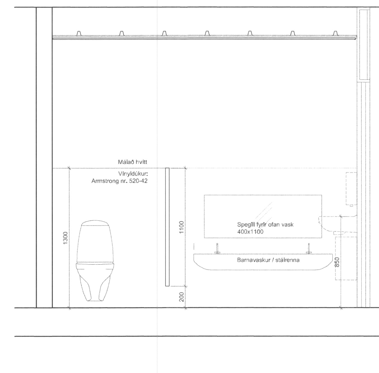
H 70/01 Sneiðing B - B, salerni 1:20
