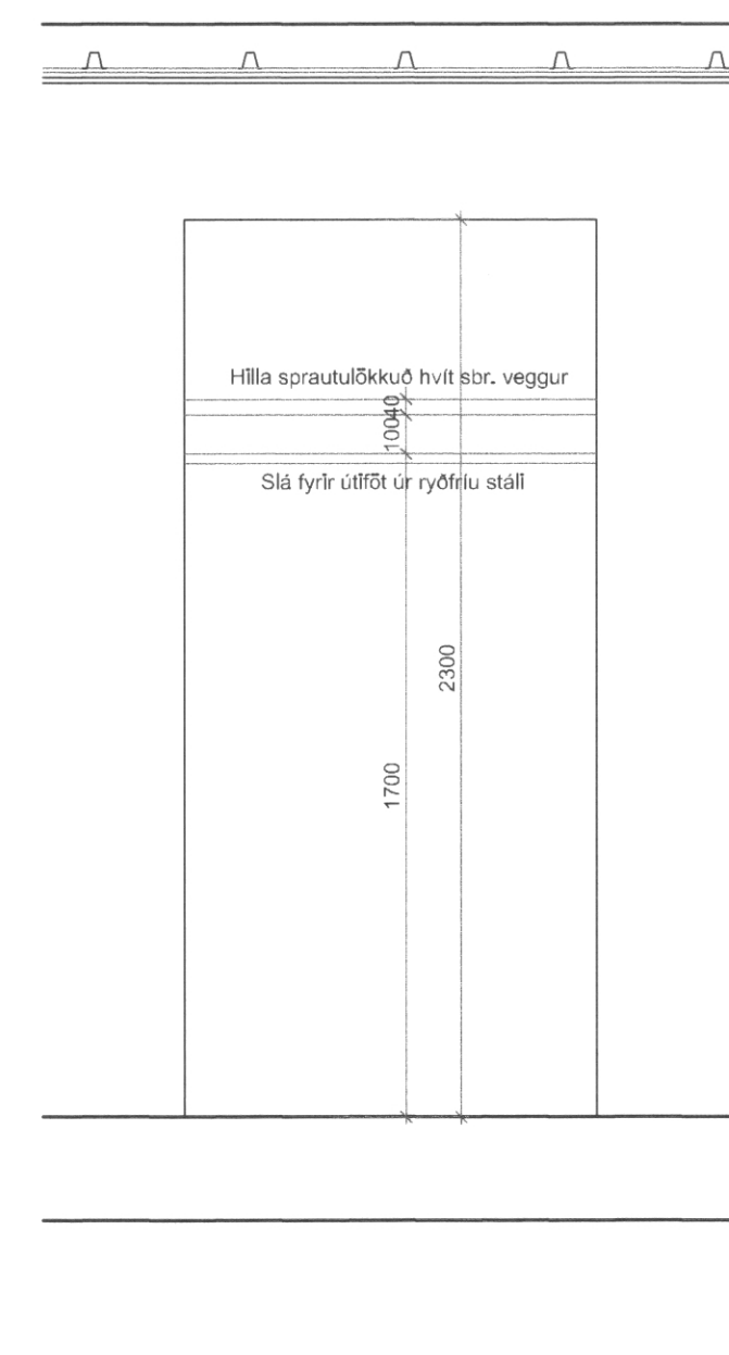
G 70/01 Sneiðing B - B, salerni 1:20
