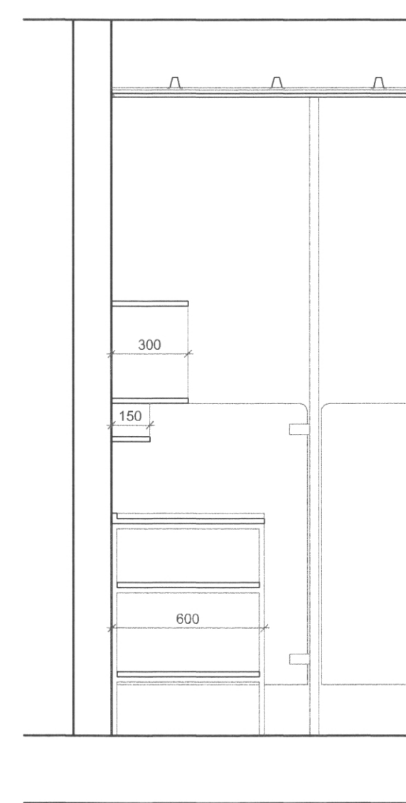
C 70/01 Sneiðing B - B, salerni 1:20
