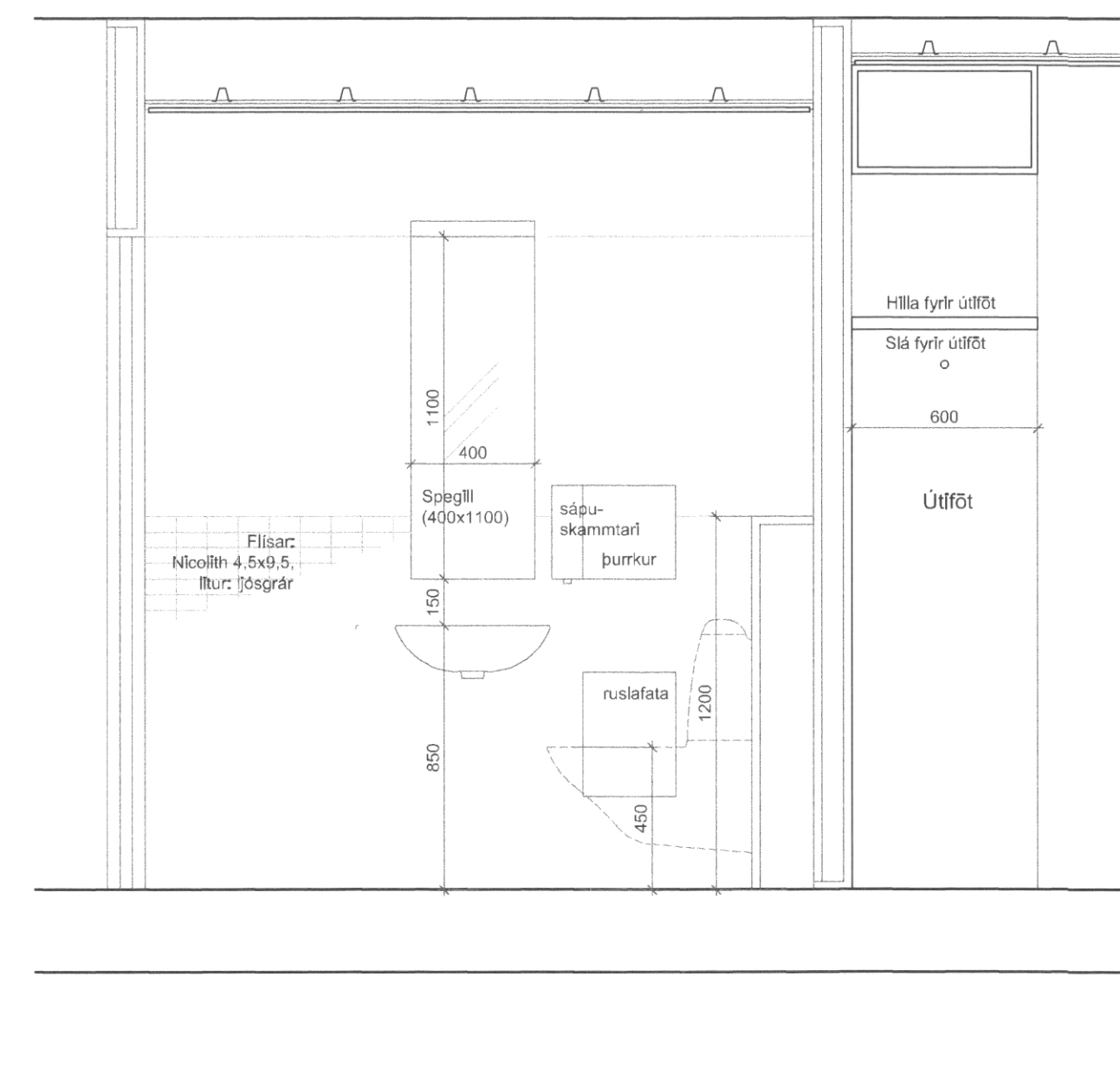
F 70/01 Sneiðing B - B, salerni 1:20
