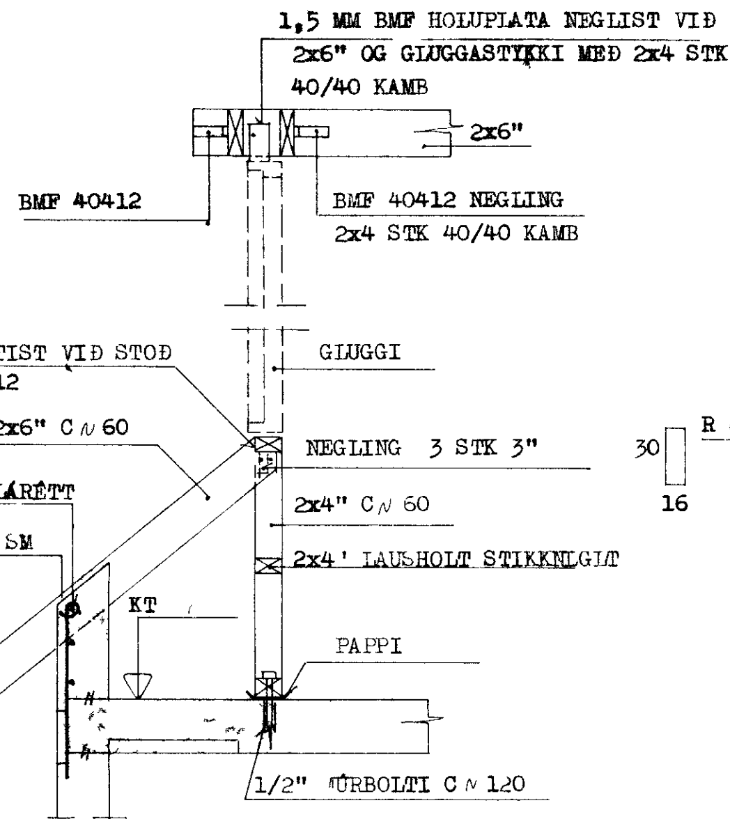
SNID F-F 1:20
