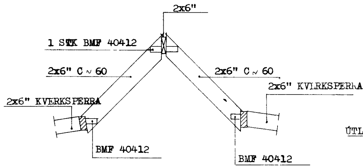
SNID E-E 1:20
